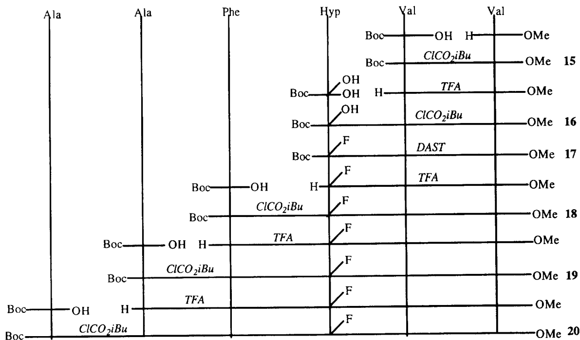
Scheme 3. Synthesis of the fluoro hexapeptide 20.
