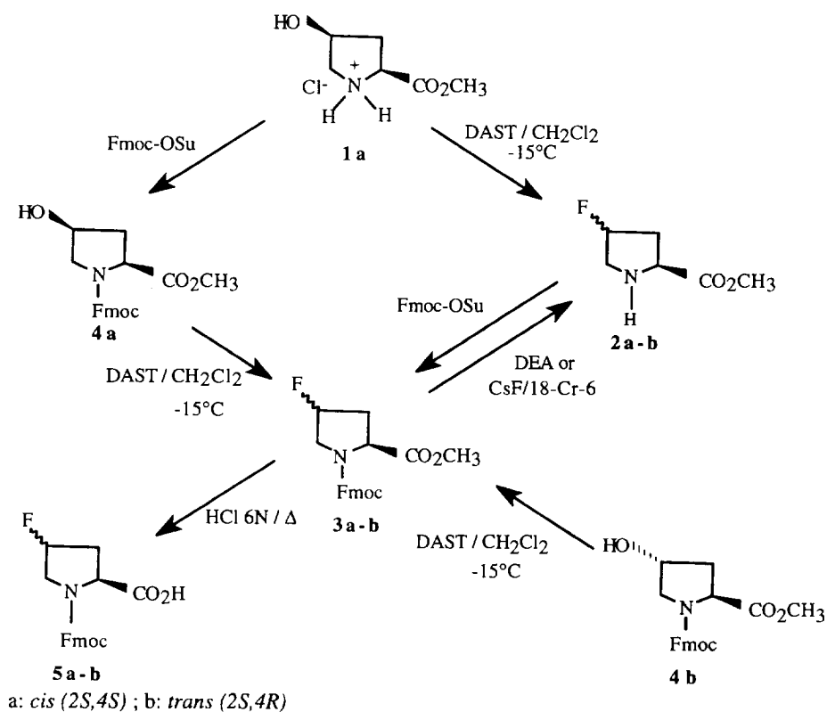
Scheme 1. Synthesis of N-Fmoc-4-fluoro-L-proline derivatives.
