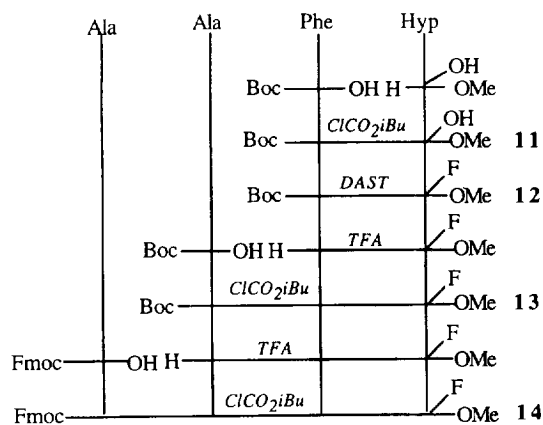
Scheme 2. Synthesis of the fluoro tetrapeptide 14.
